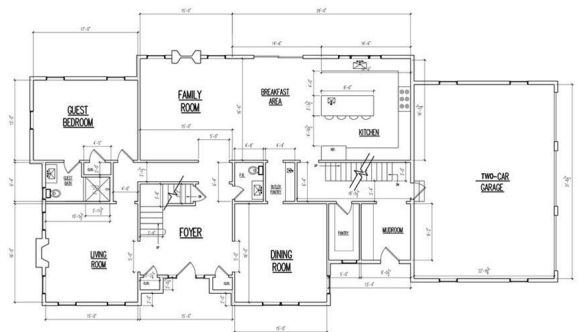
PROPOSED FIRST FLOOR PLAN 1/4" = 1'-0"
